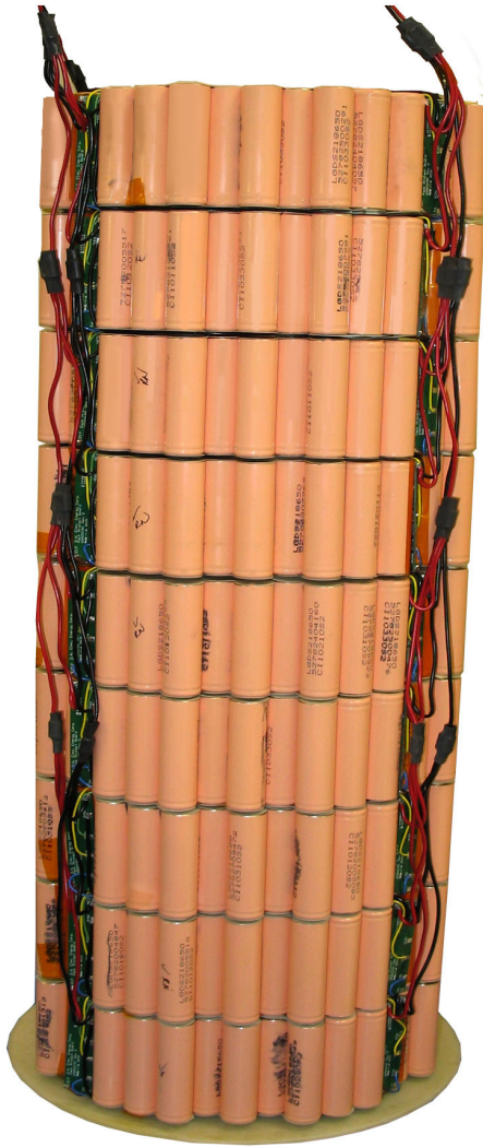
Figure 2. Early Version of a Modularly Constructed Battery Pack.
