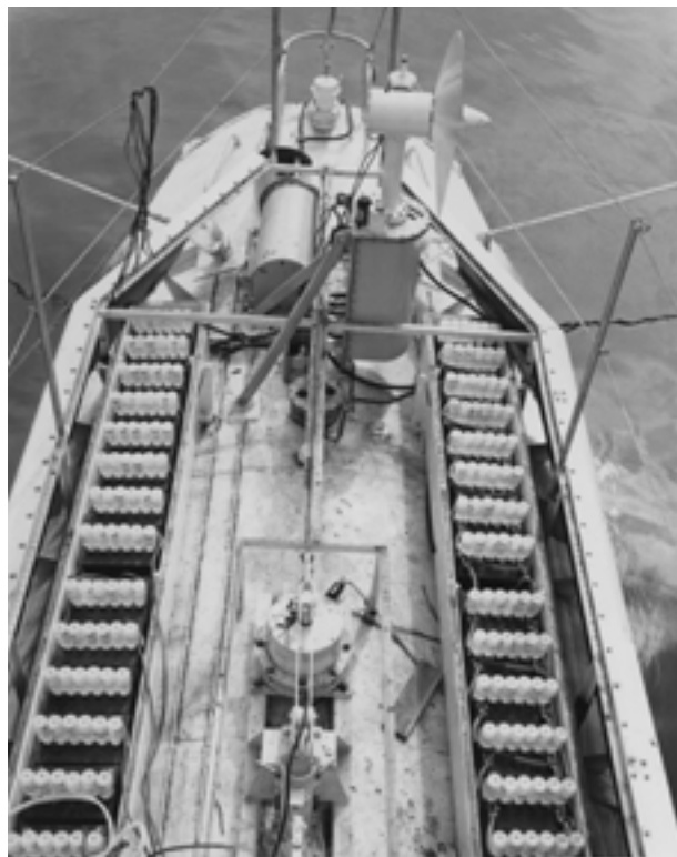
Figure 1. Trieste's pressure compensated batteries are seen in two of the four external battery boxes with the lids removed. Batteries are overfilled with electrolyte in riser pipes, then the boxes are filled with oil. A compensating system provides additional fluid to the interior as pressure increases. Also seen are two of Trieste's five pressure compensated propulsion motors, plus the emergency ballast hopper release. (Photo:
