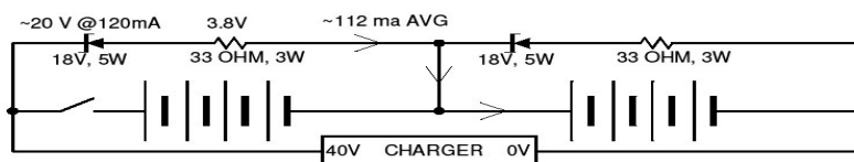
Figure 5. Zener Diode Inter-module Balancing Circuit
