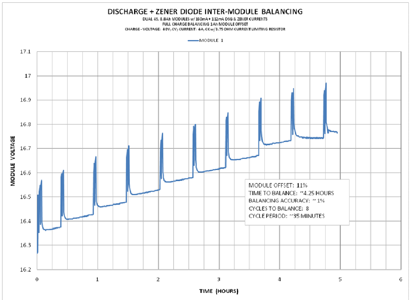
Figure 10. Combined Discharge & Zener Diode Inter-Module Balancing Example
