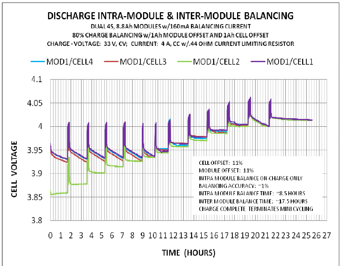
Figure 9. Combined Intra-Module & Inter-Module Balancing Example
