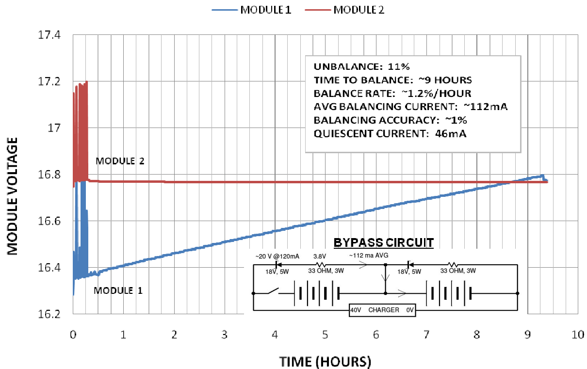
Figure 6. Zener Diode Inter-module Balancing Example
