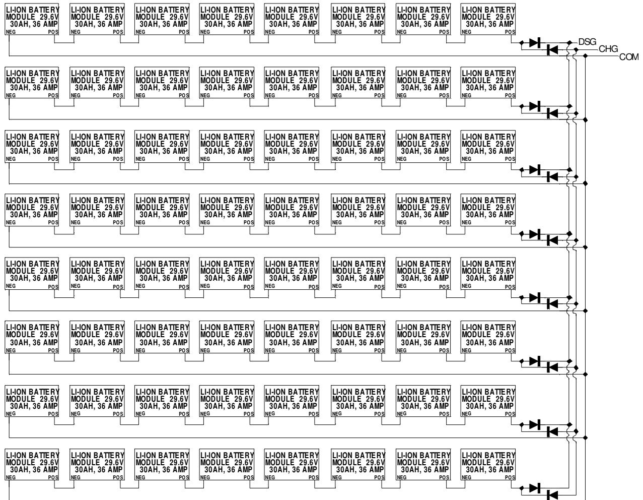
Figure 4. High Energy Battery System Constructed From Battery Modules
