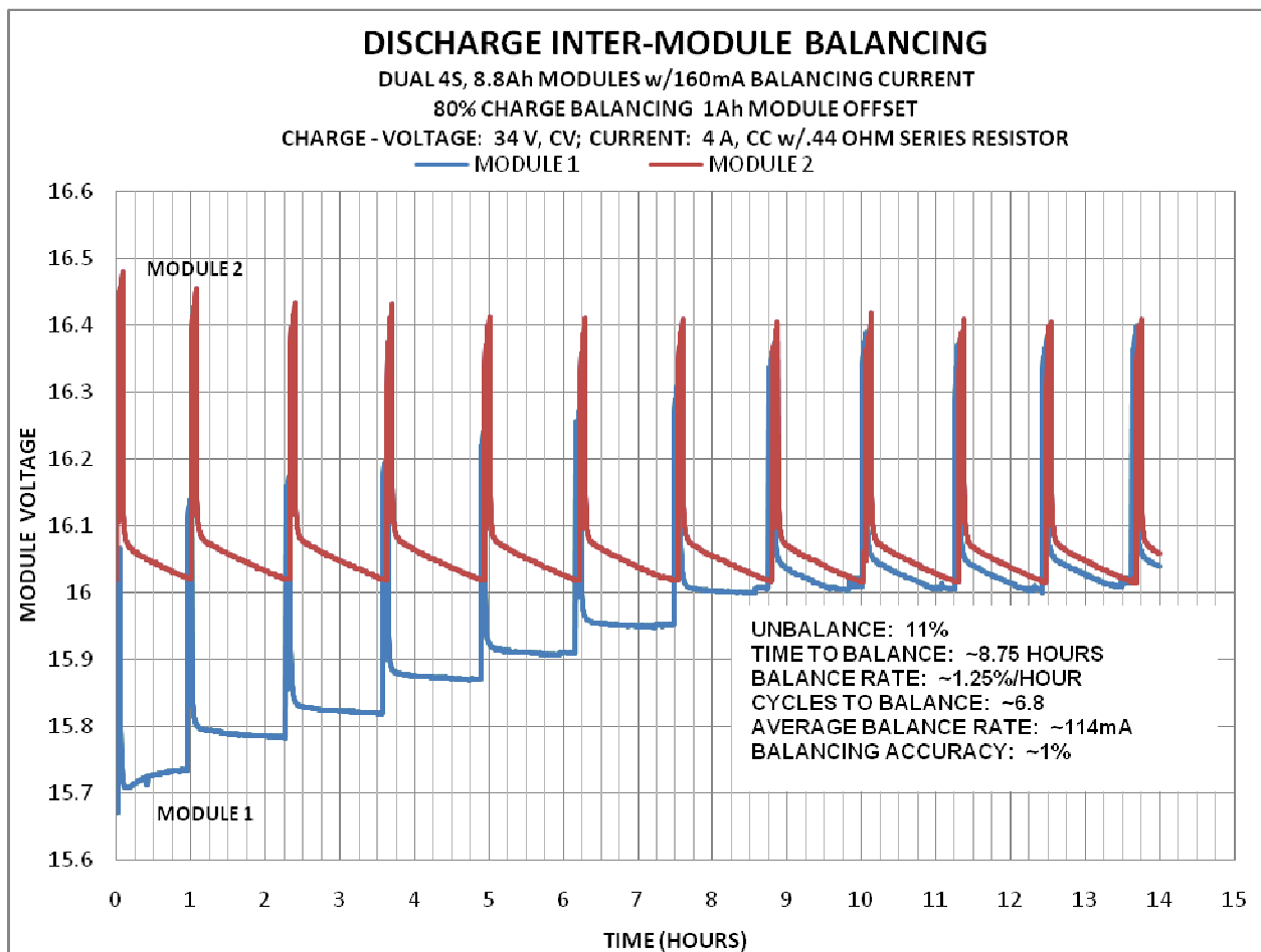
Figure 8. Discharge Module Balancing Example
