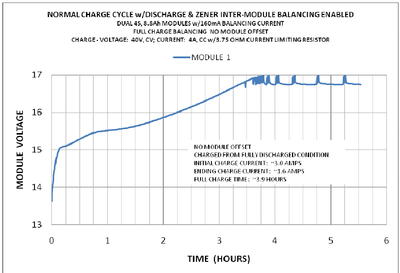
Figure 11. Example of a Full Charge Cycle When Inter-Module Balancing is Enabled
