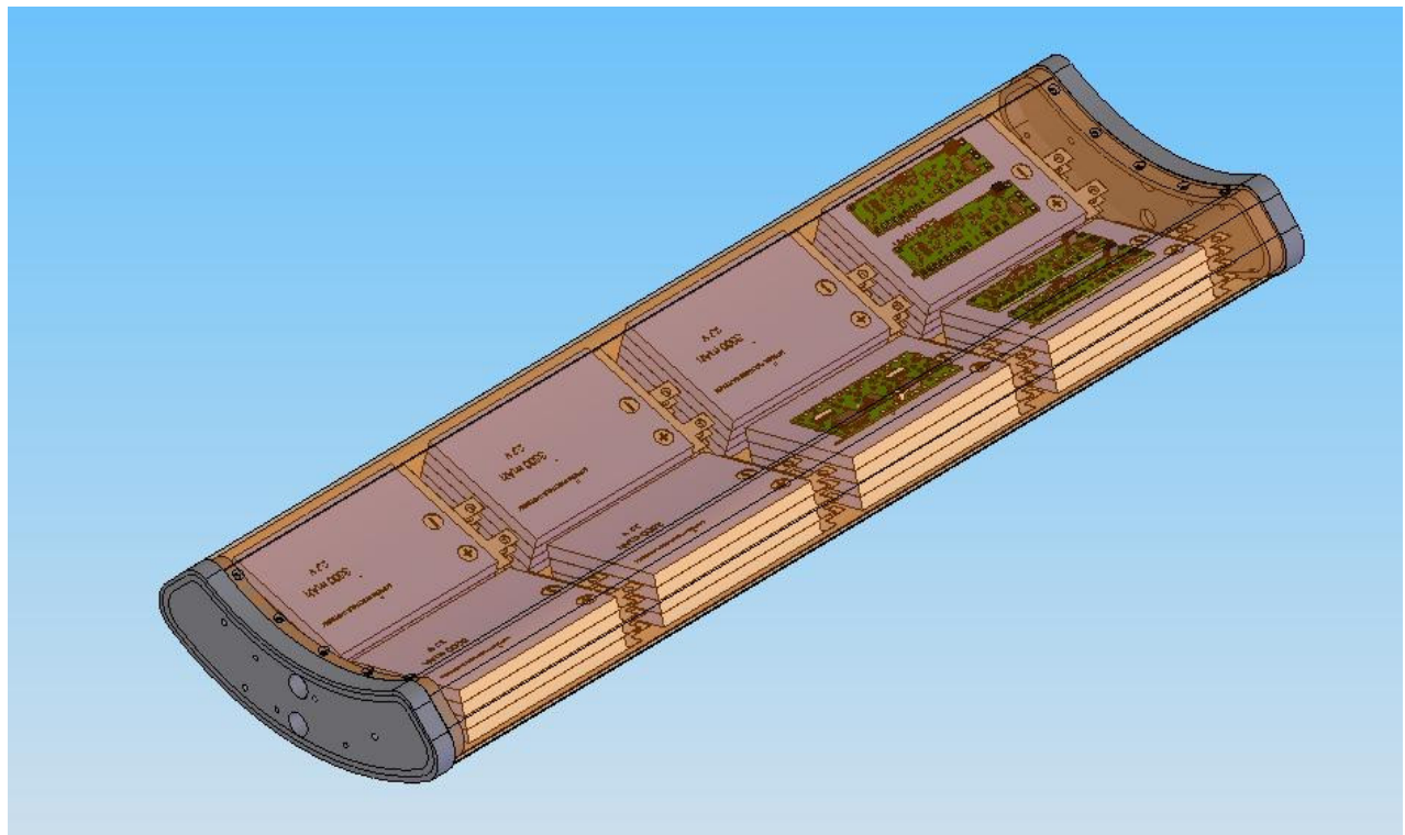
Figure 3. Illustration of a Li-Polymer Battery pack Containing 4 Battery Modules
