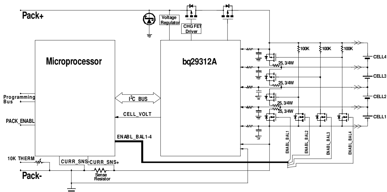
Figure 7. Discharge Intra- & Inter-Module Balancing Circuit
